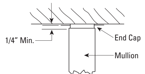
Detail G-G
